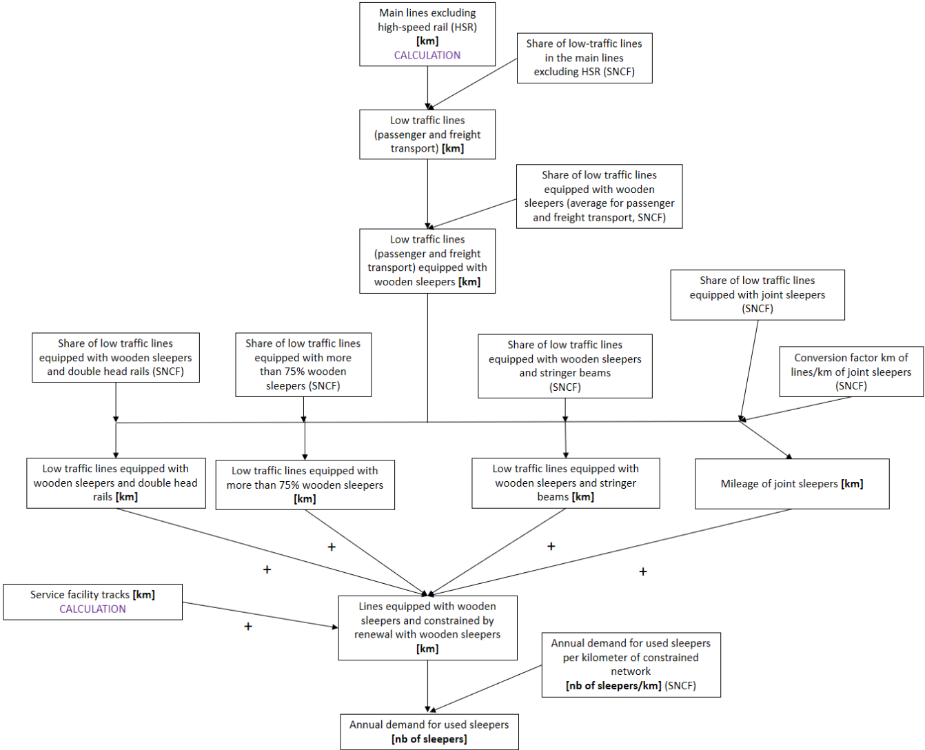
Figure B - 6: Determination of the annual demand for reusable railway sleepers - Reuse by the original user
