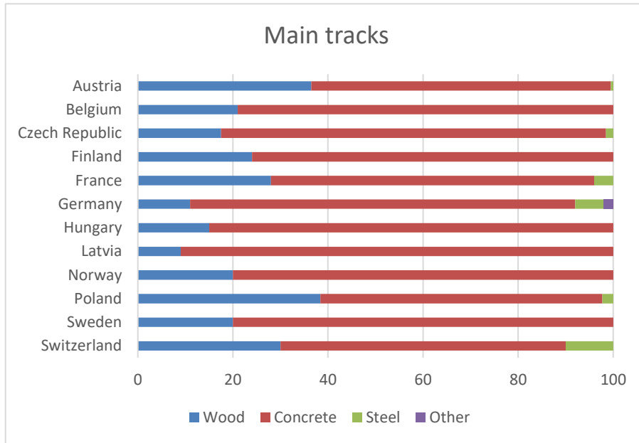
Figure B - 4: Use ratio between concrete and wooden sleepers in main tracks in European railways (figures for 2010, from UIC, 2013)
