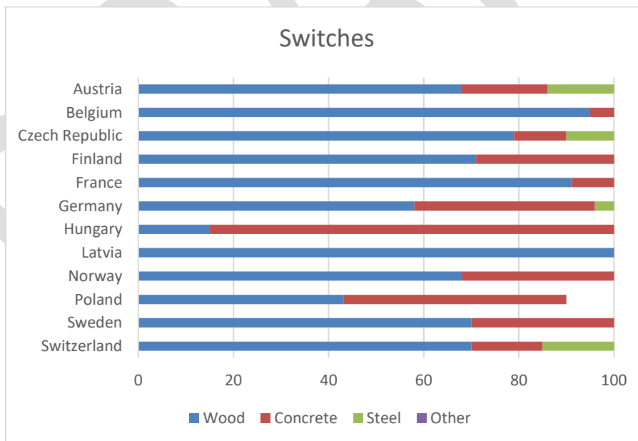
Figure B - 5: Use ratio between concrete and wooden sleepers in switches in European railways (figures for 2010, from UIC, 2013)
