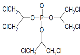
Tris[2-chloro-1-(chloromethyl)ethyl] phosphate (TDCP)
