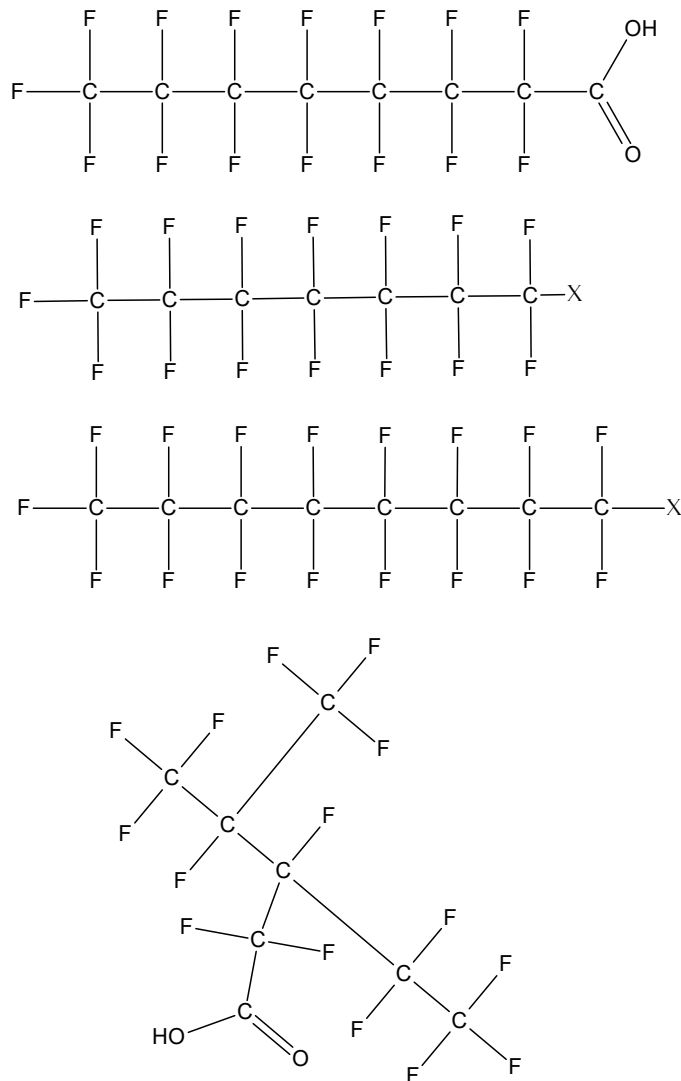
Figure A.1- 2: Chemical structure of PFOA (top) and PFOA-related substances.
