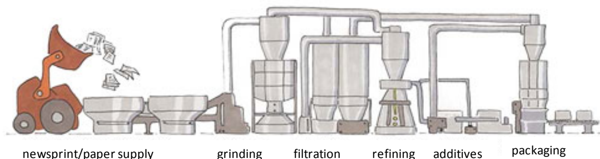
Figure 2: Cellulose insulation manufacturing (NrGaïa website, 2013)
