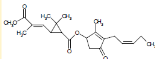
jasmolin 2
