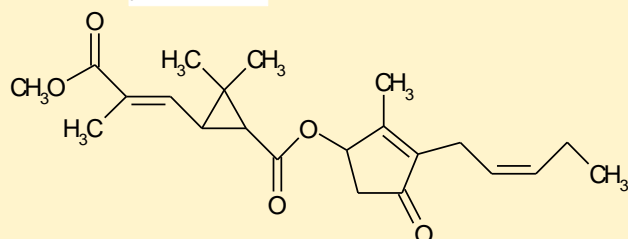
jasmolin 1
