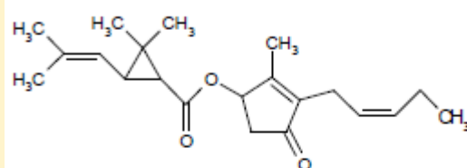
jasmolin 1
