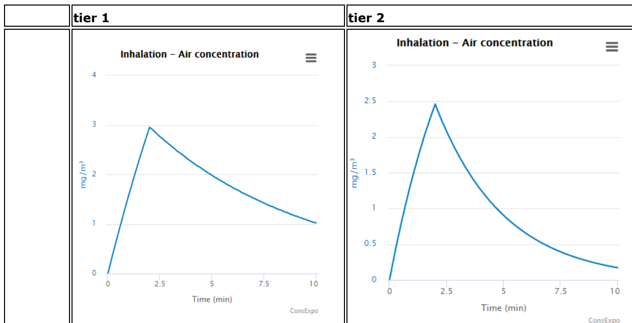
Graph II.1 Formic Acid air concentration following M&L; pharma/cleanroom
