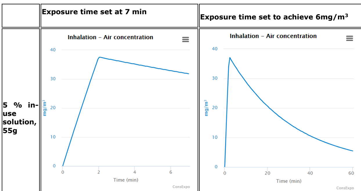
Graph II.3 Formic Acid air concentration following toilet cleaning
