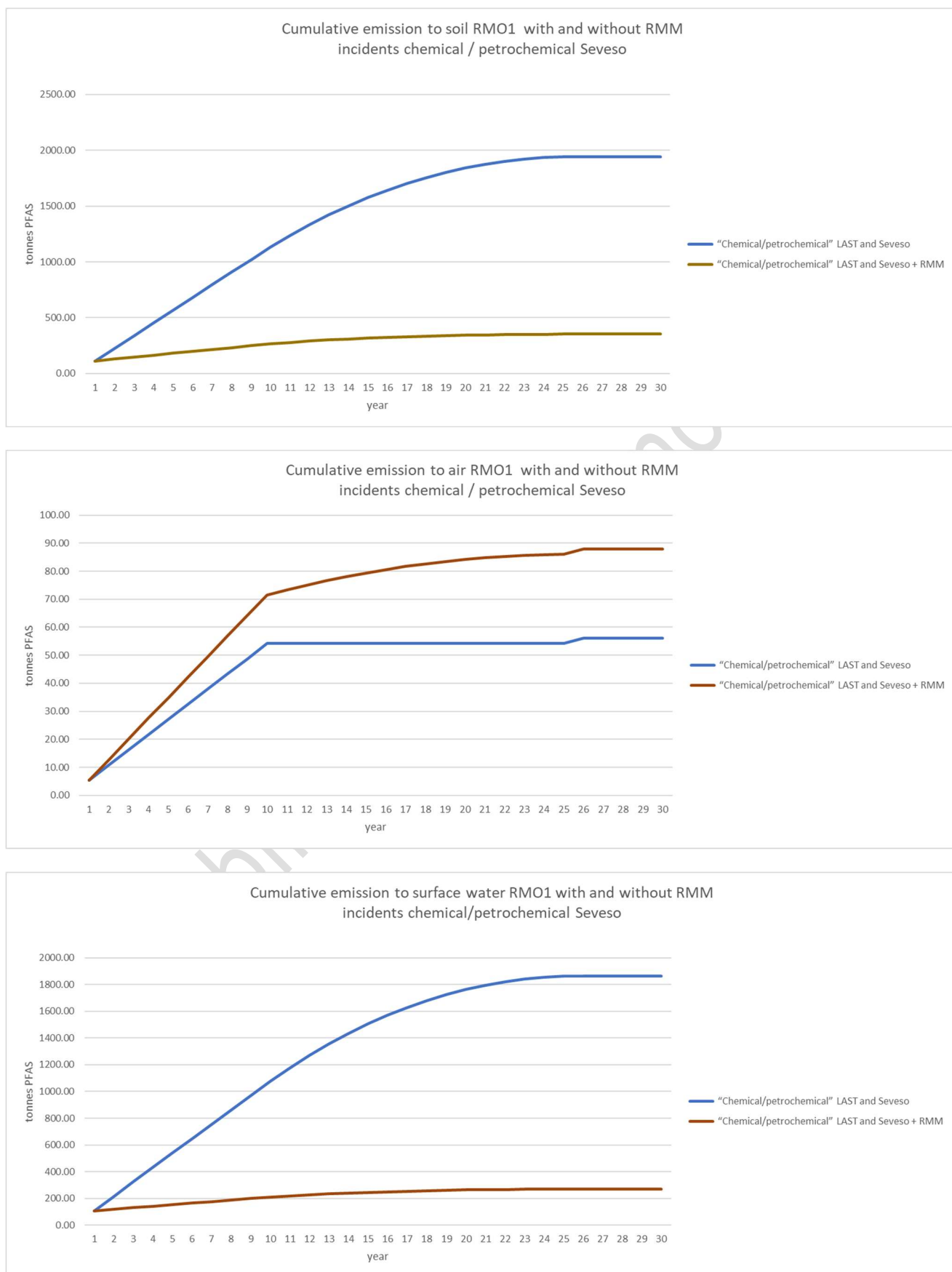
Figure 29. Cumulative emission to soil, air and surface water (t PFAS) with and without RMM for chemical / petrochemical Seveso ("Best scenario").
