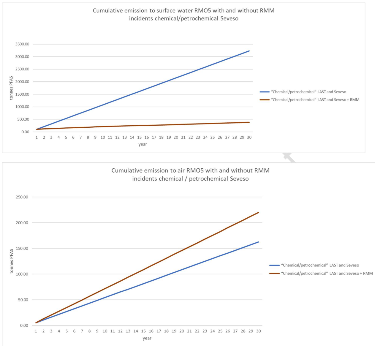
Figure 38. cumulative emissions for Seveso sector to soil, water and air under RO5 with and without RMMs.
