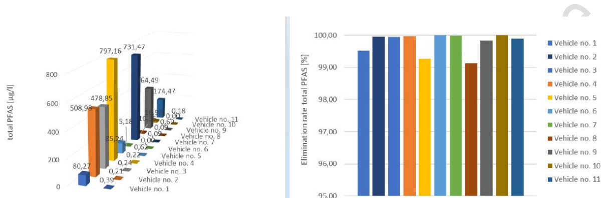
Figure 3. Results of the Cleaning of Fire Trucks using PerfluorAd.
