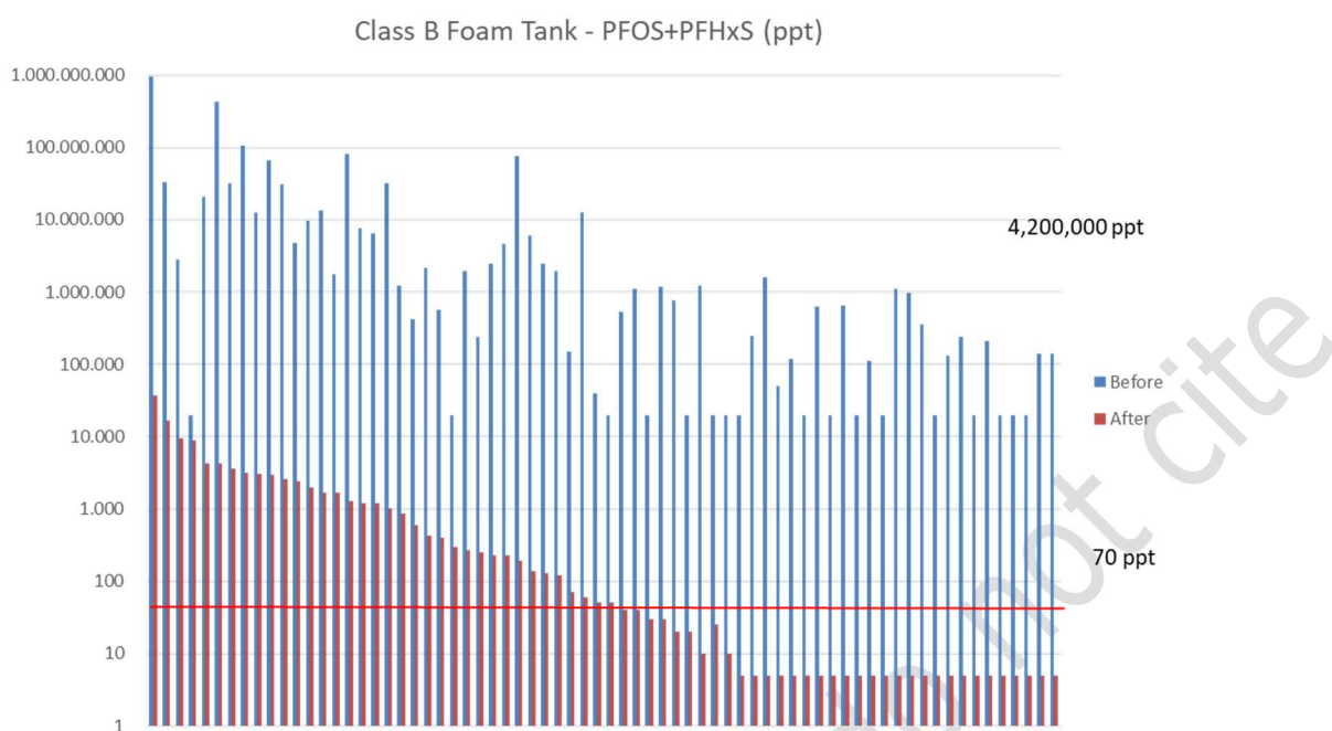
Figure 5. Achieved PFAS levels after decontamination according to the protocol by FVR, before (blue) and after (red) (taken from (Fire-Rescue-Victoria, 2021)).
